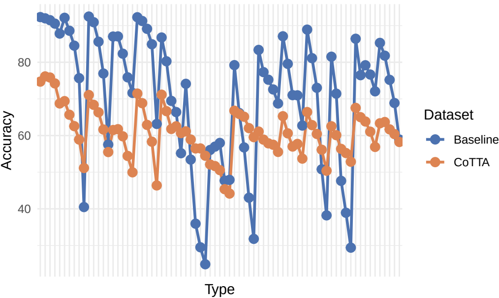
Accuracy Comparison: Baseline (No Adaptation) vs CoTTA
